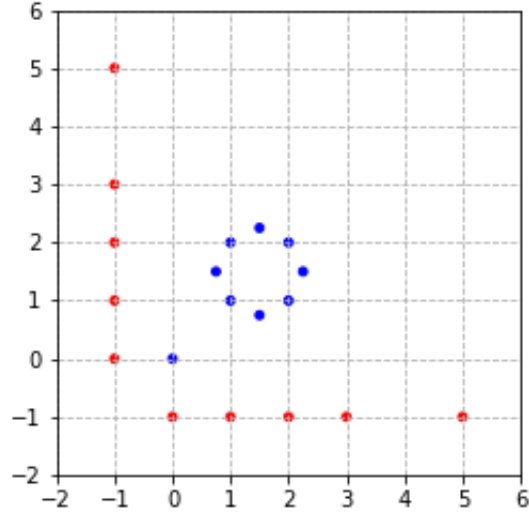
Figure 2.3: Gadget: Blue points represent set T_1 and red points represent set T_0 .
