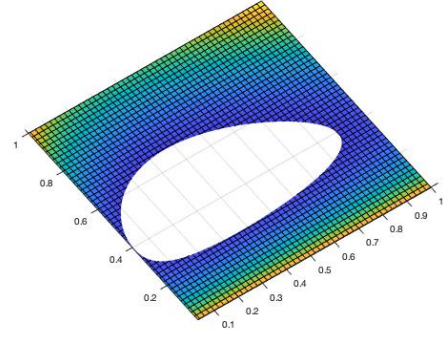
Figure 6.2: Level set \gamma(x, y) \leq -0.5
